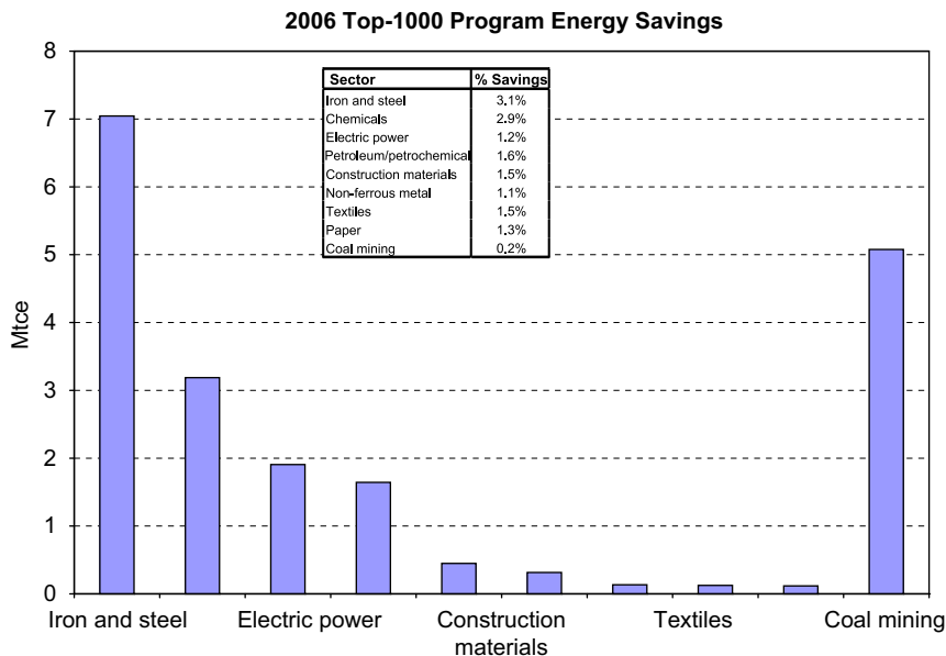
Fig. 7. A 2006 Top-1000 program energy savings. Source: NDRC and NBS, 2007.
