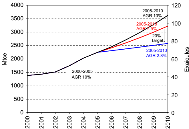
Fig. 1. Recent and projected trends in energy consumption in China, 2000–2010.
