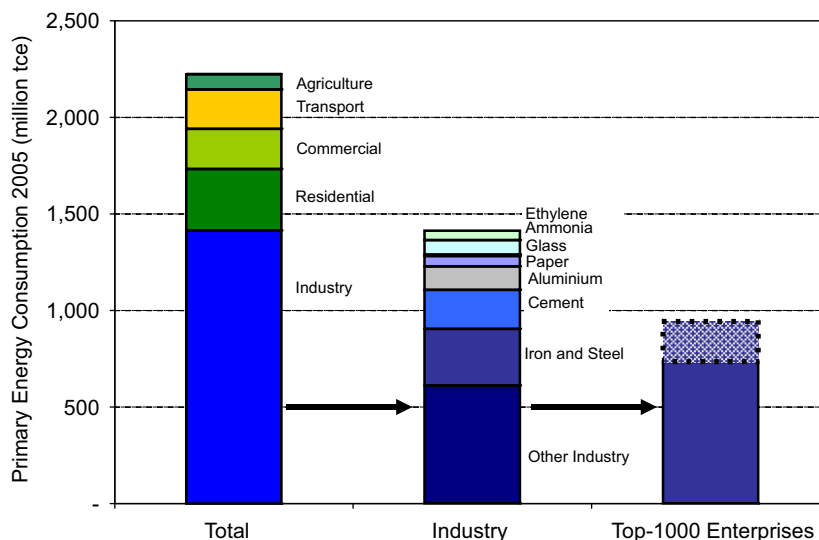
Fig. 2. Energy consumption of China, China's industrial sector, and the Top-1000 energy-consuming enterprises, 2005. Note: Top-1000 program energy consumption is typically reported in final energy units (dark blue box). The shaded area provides the Mtce equivalent of electricity generation, transmission, and distribution losses so that the Top-1000 program can be compared in primary energy terms with the other two bars. Industry sub-sector breakdown based on LBNL LEAP model, not Chinese statistics. (For interpretation of the references to colour in this figure legend, the reader is referred to the web version of this article.)
